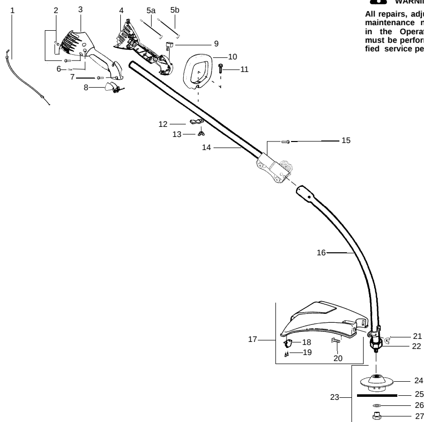
SEARS TRIMMER MODEL 944.511561
